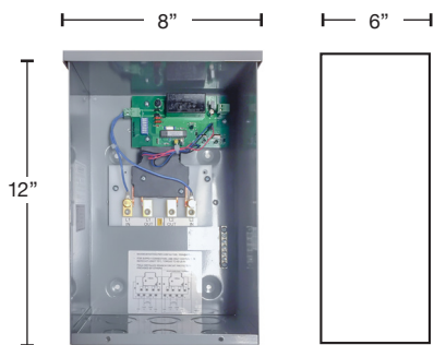
1-Phase 100A Latching Relay
