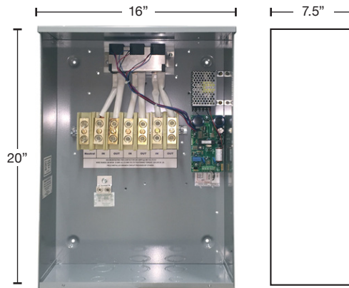
3-Phase 200A Latching Relay
